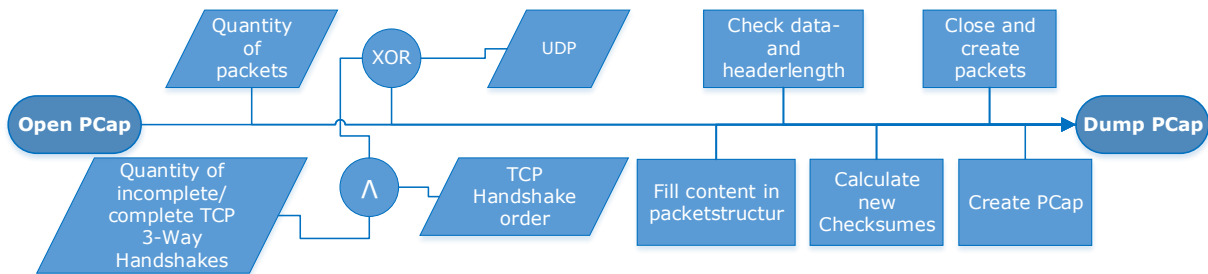
Figure 2: Creating PCap
