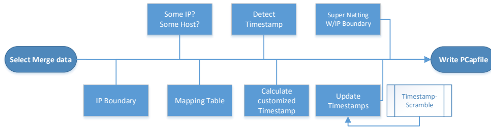
Figure 1: PCap merging
