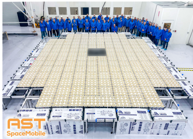
FIGURE 6. Unfolded BlueWalker 3 [7].
