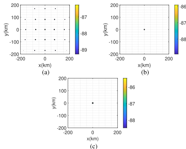
FIGURE 16. Beam pattern projection on a 400 \times 400 km Earth surface: (a) URA with grating lobe problem, (b) LSA, (c) ELSA ( st_c = 0.1 ).
