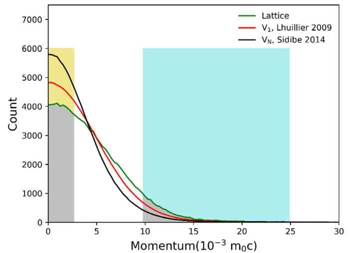
Fig. 10. The averaged DB spectrum from 6 to 25 keV for the largest vacancy cluster V_N and single vacancy V_1 in comparison with that of pristine one obtained for 25 keV slow positron. The windows for line-shape parameters S and W are also illustrated. The V_1 and V_N curves are from Ref. [48] and Ref. [52], respectively.
