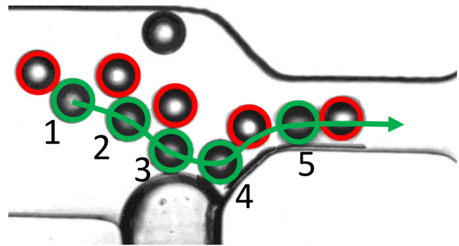
FIG. 5. In frames 1–4, the bubble is excited, causing two particles (labeled green and red) to be drawn near the bubble’s surface. If the excitation continues, these two particles will remain in the positions depicted in frame 4 until additional particles push them toward the exit. In the current scenario, however, the microbubble is deactivated after frame 4, allowing the main flow to carry the particles to the exit through the throat.
