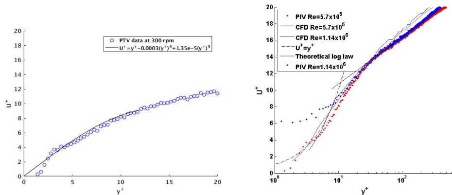
(a) Viscous sublayer region velocity profile from PTV measurements compared with theoretical mean velocity profile
