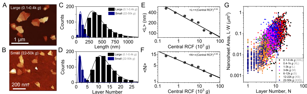
Figure 1. AFM statistics on fractions of size-selected \alpha - \text{RuCl}_3 : (A), (B) AFM images of drop cast nanosheets for two fractions containing relatively large, ((A), 0.1–0.4k g) and small ((B), 22–50k g) nanosheets. (C), (D) histograms of lateral sheet size (C) and layer number (D) distribution for the two fractions shown in (A) and (B). The histograms for the large fraction are depicted in black, the histograms for the small fraction in blue (for the other fractions see SI, figure S4). (E) Mean lateral size of nanosheets across all fractions on a double logarithmic scale. Note, that we define the length as the longest dimension of a sheet. (F) Mean layer number of nanosheets across all fractions on a double logarithmic scale. The AFM apparent height is converted into layer number by step height analysis on terraces on the sheets (see SI, figure S3 for details). The solid lines are linear fits, highlighting the power law dependence for both, \langle L \rangle and \langle N \rangle with the central centrifugation speed between two steps. (G) Scatter plot of the nanosheet area (product of length and width) as a function of their layer number across the different fractions of the size selection.
