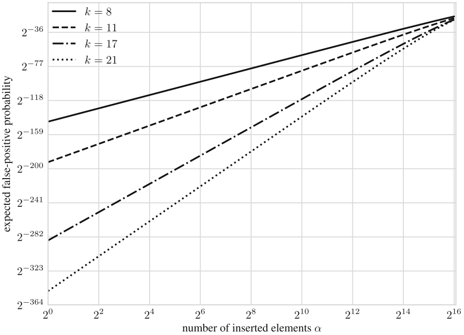
Fig. 9. The false-positive probability of a random element after \alpha elements have been added to a Bloom filter with n = 2^{16} for k \in \{8, 11, 17, 21\} .
